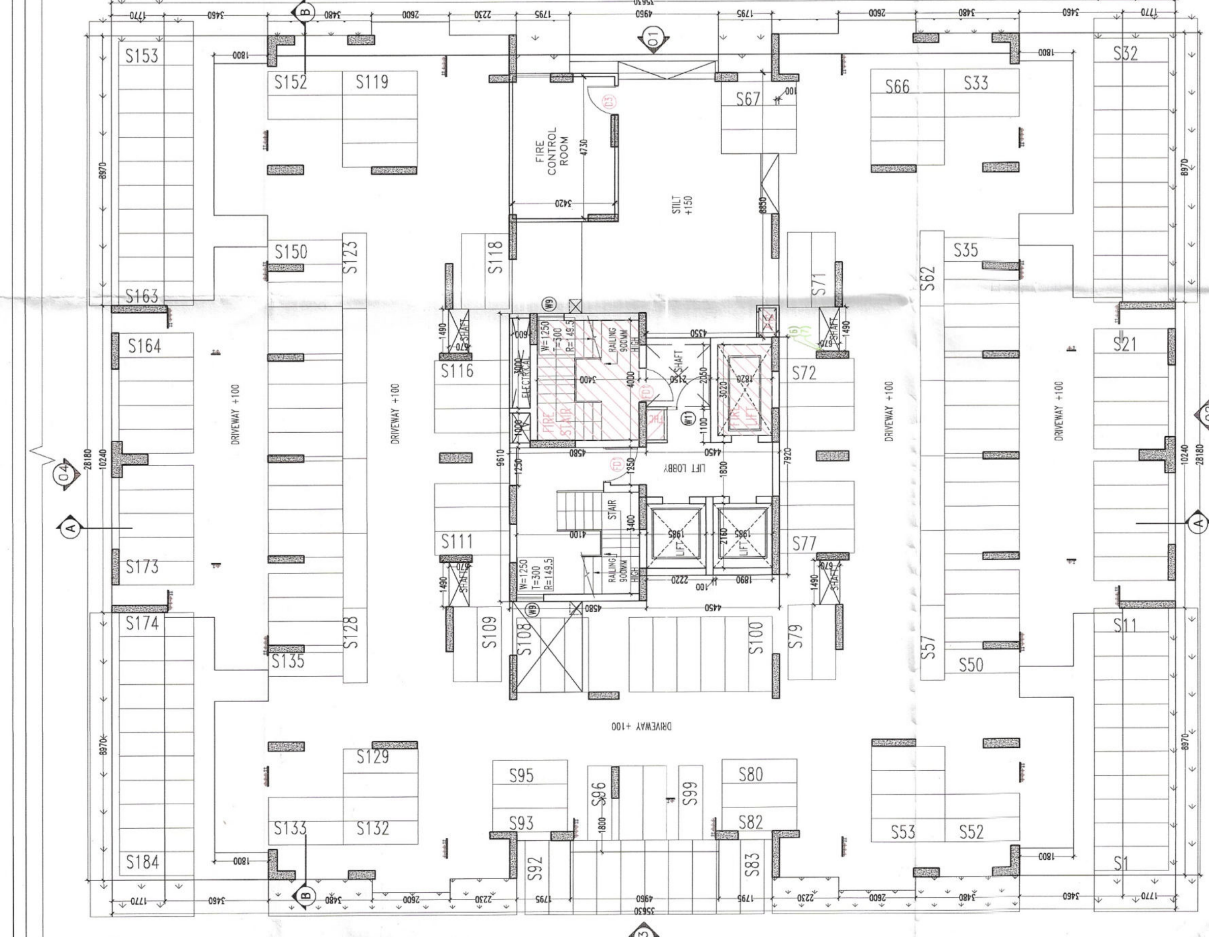
STAIR/GROUND FLOOR PLAN TOILET DETAILS ARE TYPICAL (REFER DWG NO. 16)
