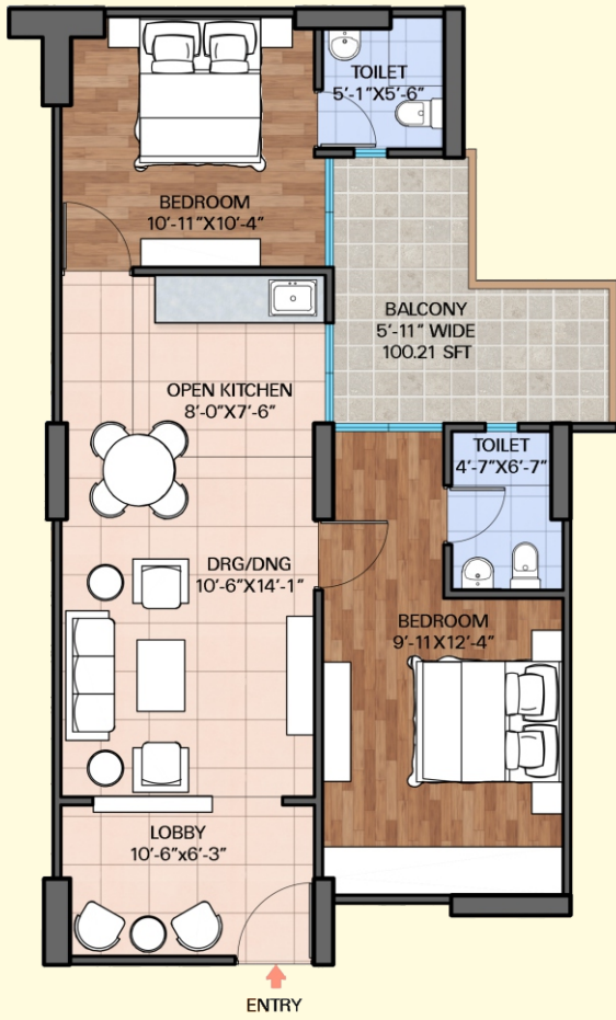
UNIT TYPE - 1
